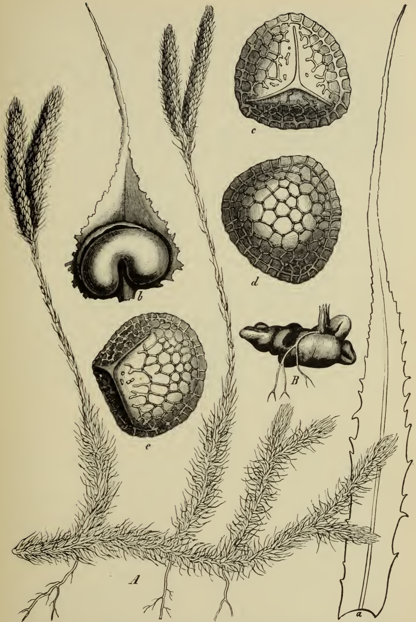
FIG. 26.— Lycopodium . A , portion of Lycopodium clavatum , Linn. (natural size); a , foliage leaf; b , sporophyll, with sporangium, magnified; c , d , e , spores magnified about 600 diameters; B , prothallium of an allied species. (Luerssen.)
